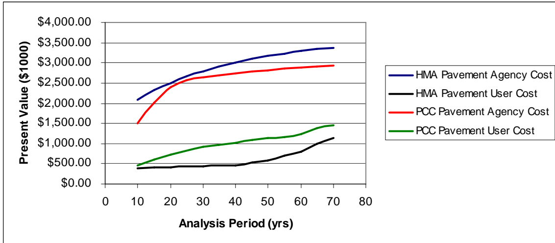
Figure E-5 The effect of analysis period on agency and user costs – remaining service life and 3% discount rate
