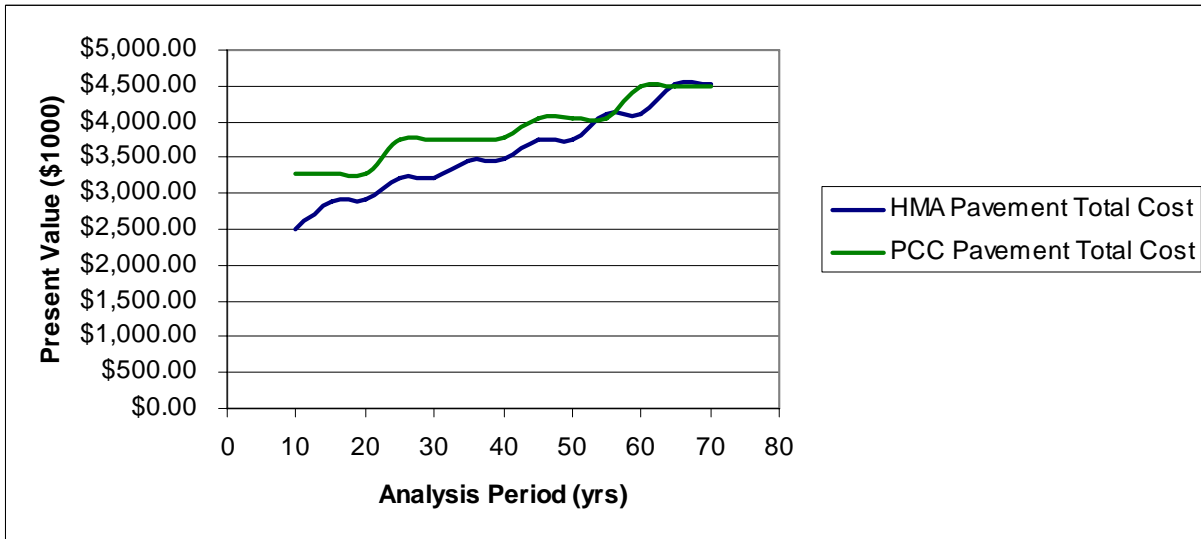
Figure E-10 The effect of analysis period on total cost – no remaining service life and 3% discount rate
