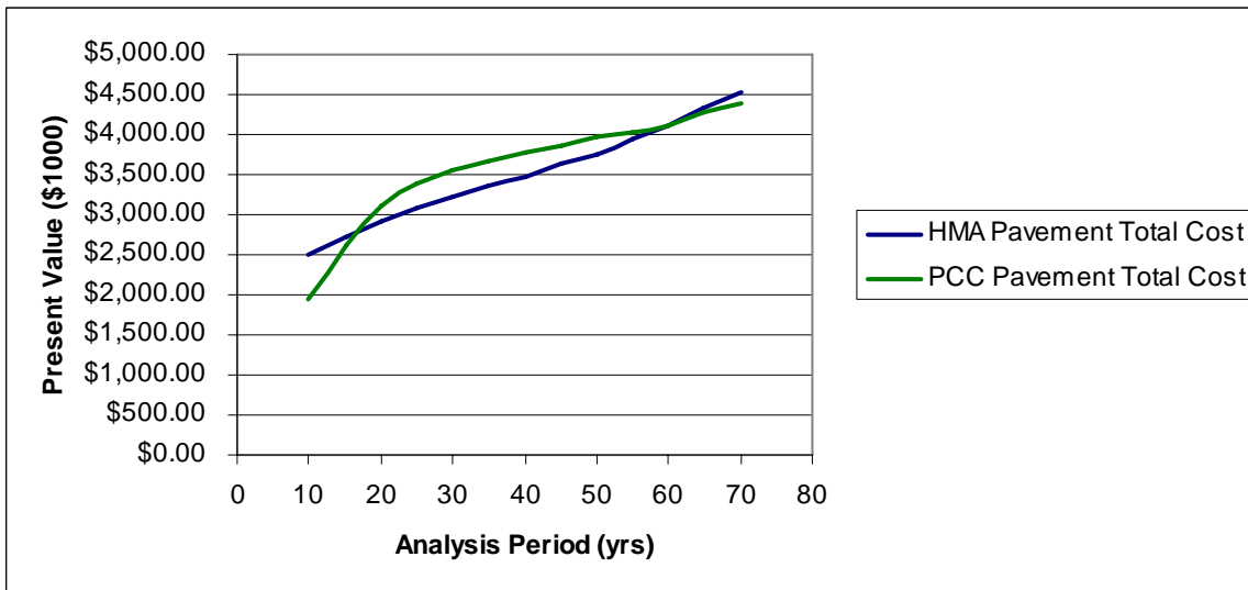
Figure E-6 The effect of analysis period on total cost– remaining service life and 3% discount rate
