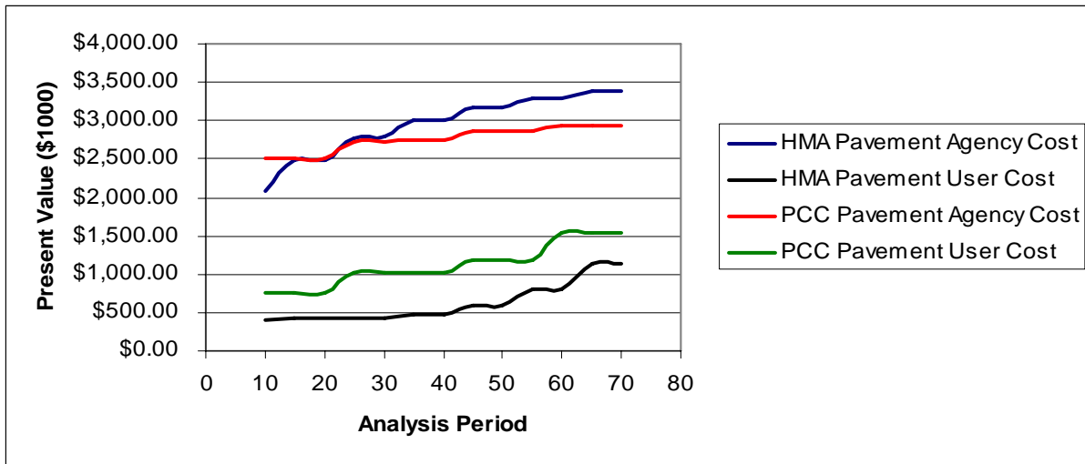
Figure E-9 The effect of analysis period on agency and user costs – no remaining service life and 3% discount rate
