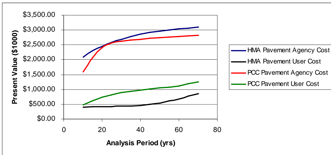
Figure E-3 The effect of analysis period on agency and user costs– remaining service life and 4% discount rate
