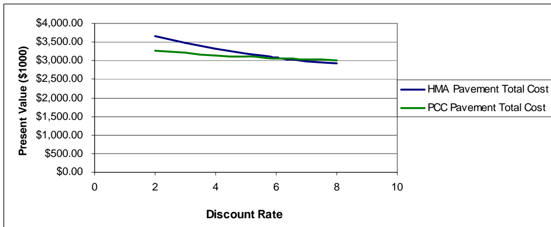
Figure E-2 The Effect of Discount Rate on Total Cost
