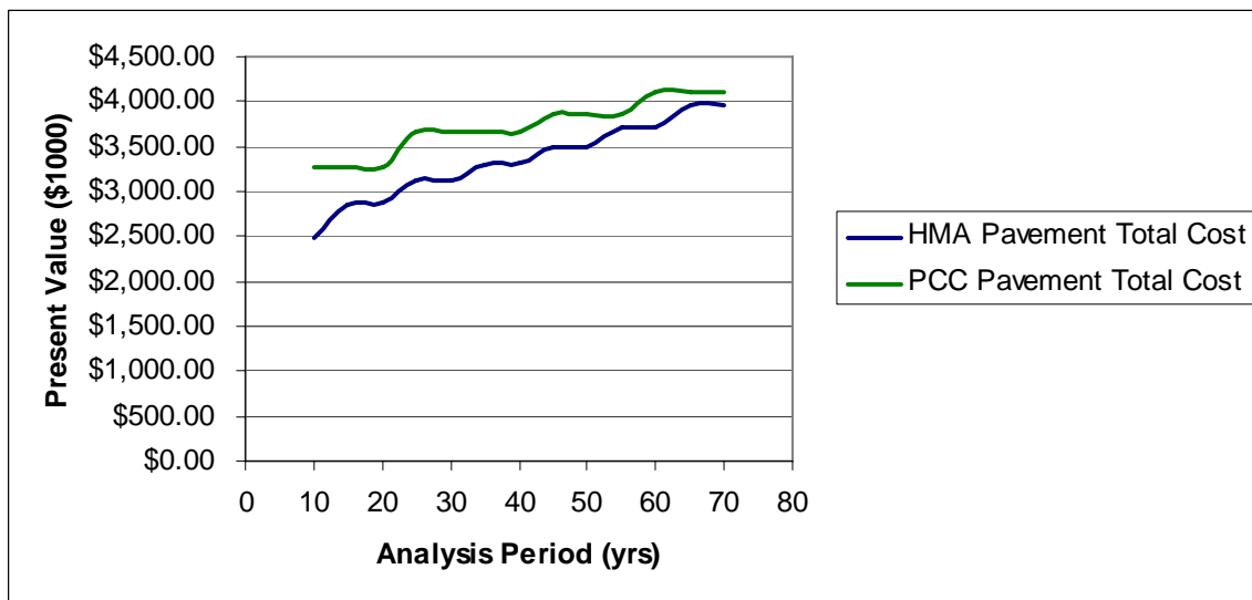
Figure E-8 The effect of analysis period on total cost – no remaining service life and 4% discount rate
