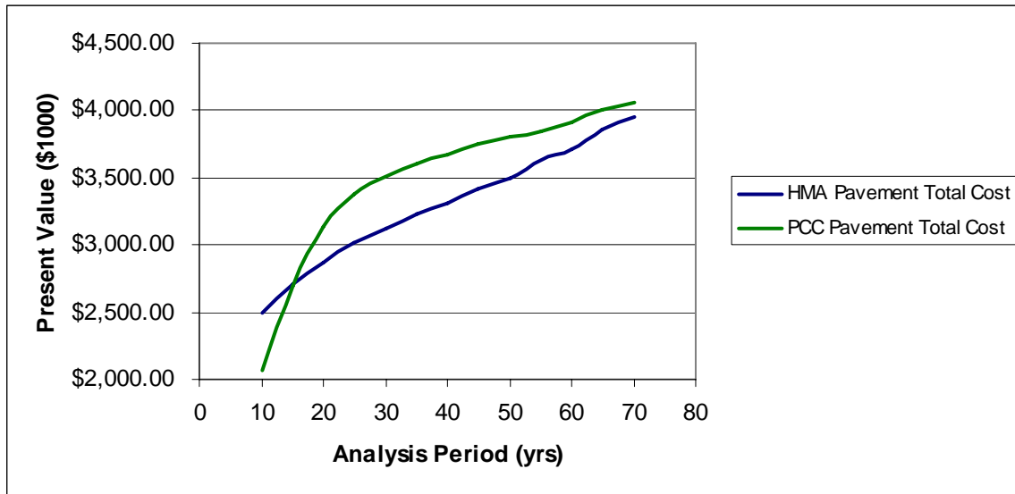
Figure E-4 The effect of analysis period on total cost costs – remaining service life and 4% discount rate
