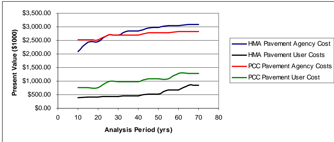
Figure E-7 The effect of analysis period on agency and user costs – no remaining service life and 4% discount rate
